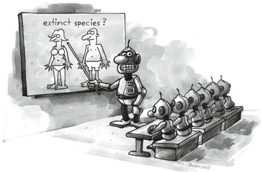
Fig. 8.1 Supervised learning ...
