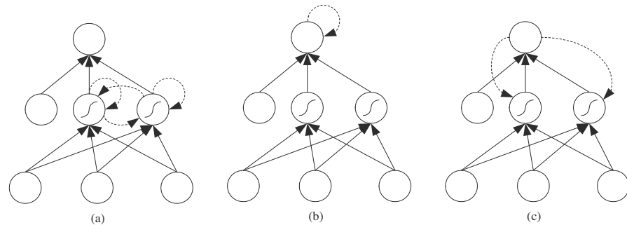
Figure 11.21 Examples of MLP with partial recurrence. Recurrent connections are shown with dashed lines: (a) self-connections in the hidden layer, (b) self-connections in the output layer, and (c) connections from the output to the hidden layer. Combinations of these are also possible.
