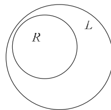
(b) Precision = 1
