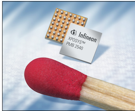
FIGURE 6-3: GPS chips turn tiny.
